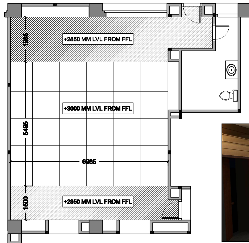
REFLECTED CEILING PLAN LAYOUT
