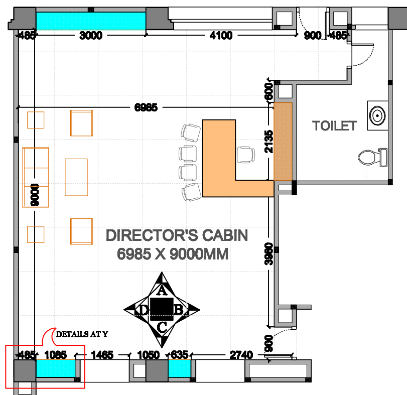
FURNITURE LAYOUT OF THE DIRECTOR'S CABIN-6
