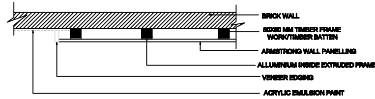
DETAILS AT 'X'
