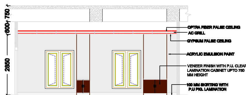
ELEVATION AT C
